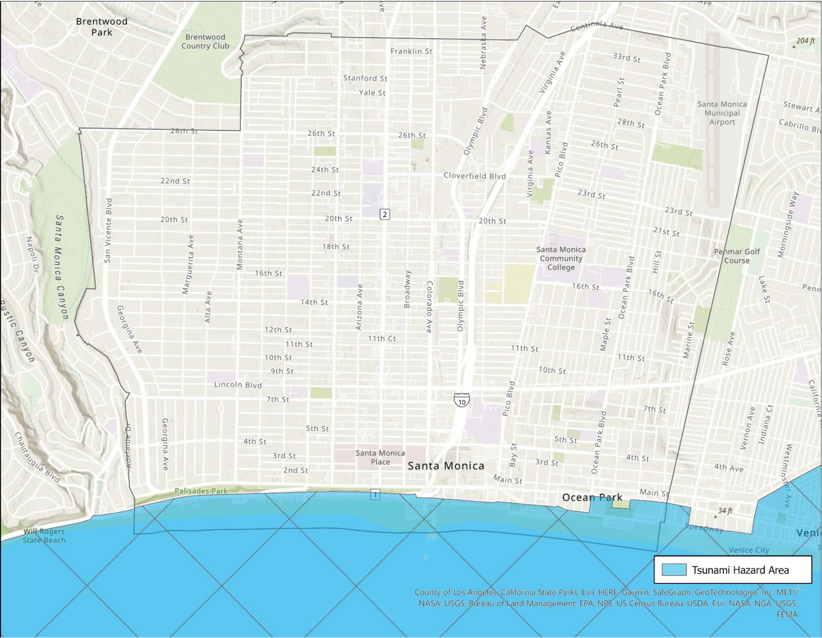
Figure 6 - Tsunami Hazard
