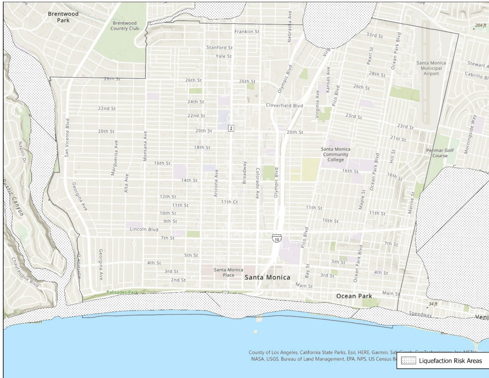
Figure 4 - Liquefaction Risk
