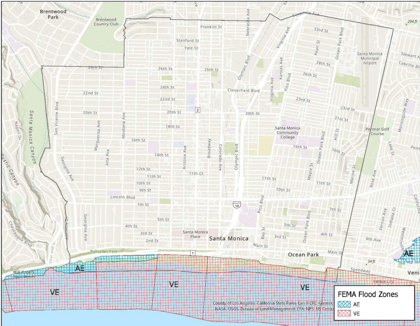
Figure 5 - Flood Zones
